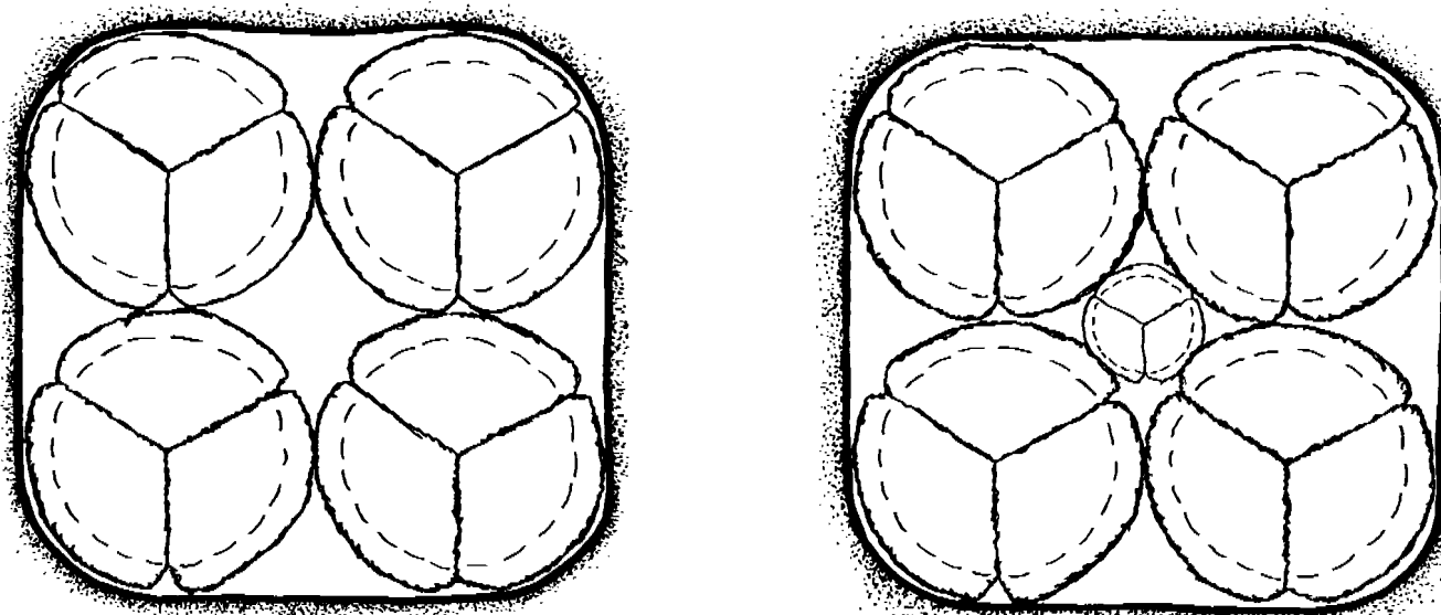
Figure 12.56. A square rope-hole suggests that it was intended for four (A) or even five (B) smaller cables instead of one large cable (drawn by the author)
