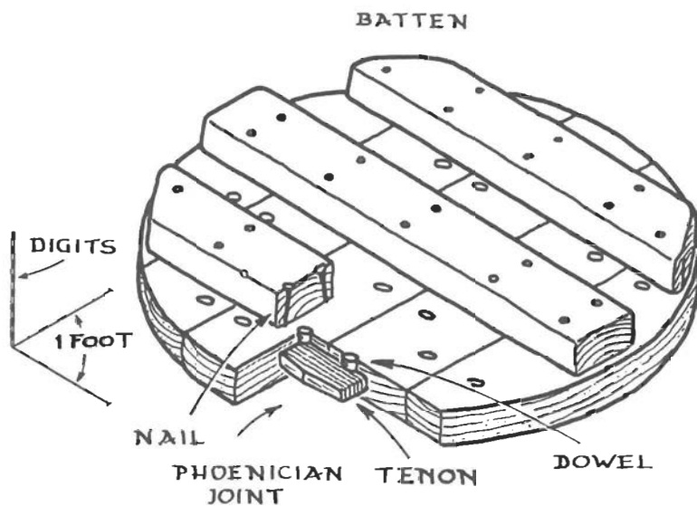
Figure 10.30. Schematic reconstruction of Cato's oil-press disk ( orbis olearium ) with "Phoenician joints" (courtesy A. W. Sleeswyk)
